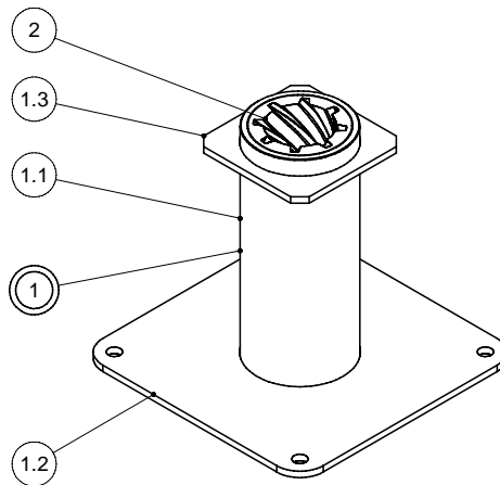
BEARING KIT 550-02-00-000
